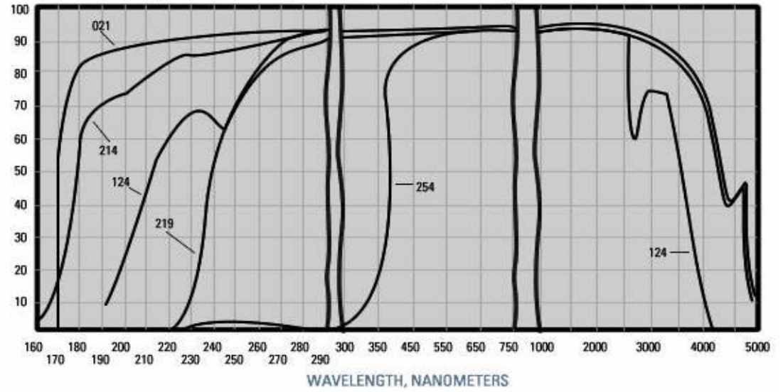
Fused Quartz Average Transmittance Curves
