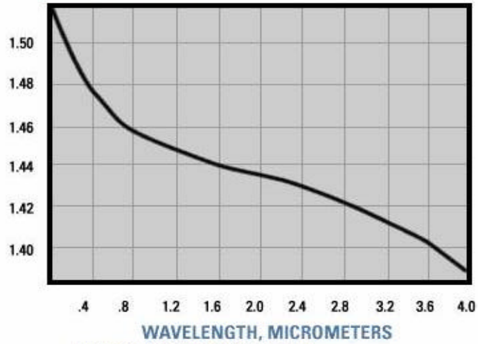
Index of Refraction
